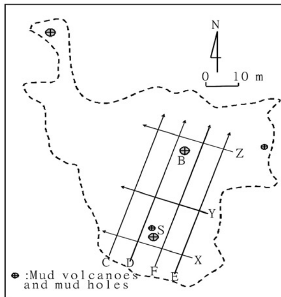
Figure 2. (a) Satellite image of the WNLPA (from Google TM earth) and pictures of the mud volcano B (upper left) and mud volcano S (lower right). (b) Resistivity survey plan of the WNLPA site (dotted line indicates the range of the WNLPA). B and S mark the locations of two major mud-volcano craters. Resistivity surveys were conducted along the C, D, E, and F lines and along the X, Y, and Z lines. Arrows show the survey direction.
