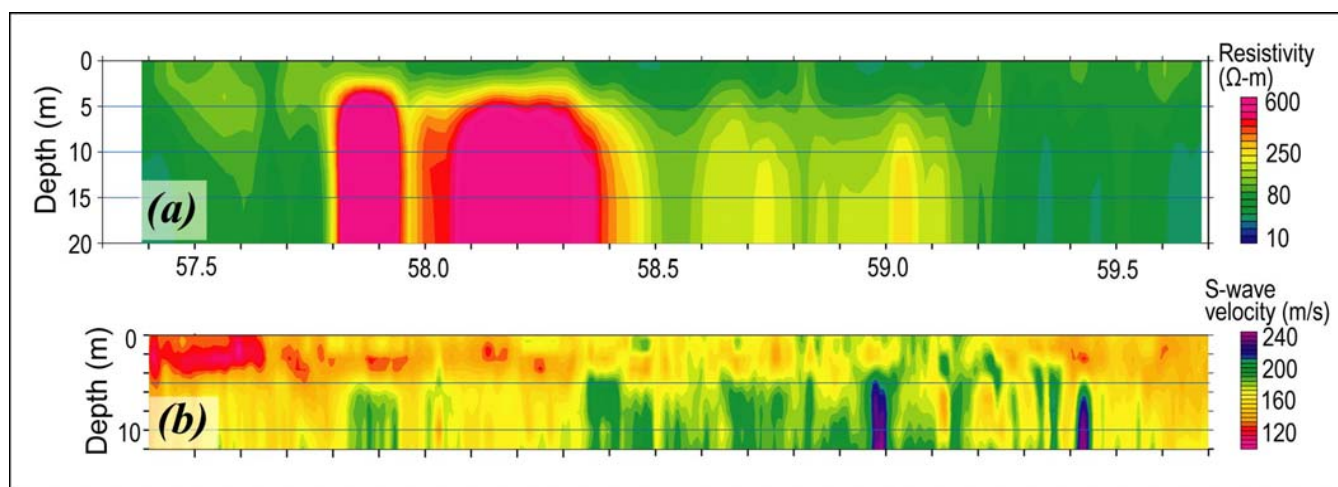
Figure 8. A resistivity (a) and S-wave velocity (b) profile along the levee at Edo_58L site. A high resistivity anomaly was delineated at the portion from 57.8 to 58.4 km, whereas the S-wave velocities at the anomaly were not so high. The upstream part of the line (59.2 to 59.7 km) showed relatively low resistivity and relatively low S-wave velocity.
