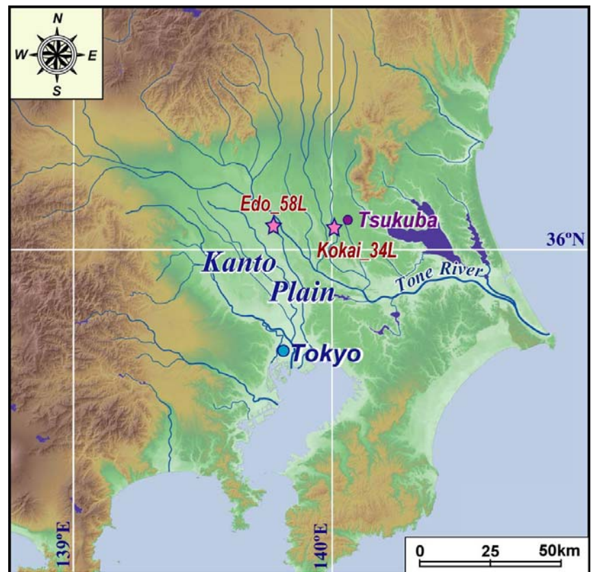
Figure 2. Map showing test sites. Integrated geophysical surveys were conducted on earthen levees along Edo and Kokai River, both are the branches of Tone River which flows through the Kanto Plain, central Japan.
