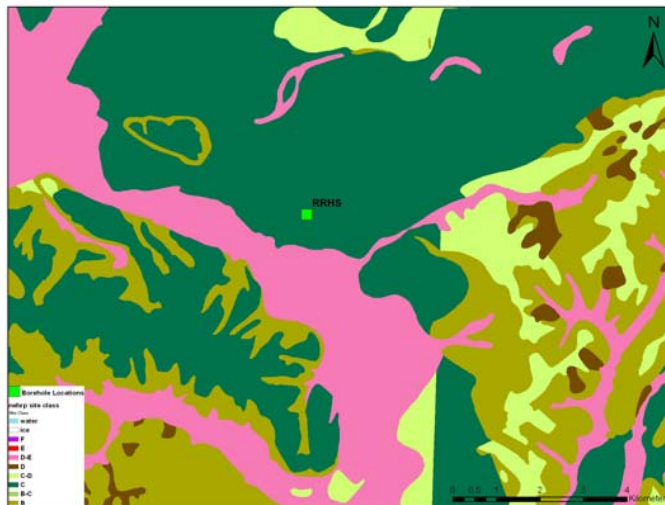
Figure 5: RRHS site (green square) is underlain by NEHRP site class map (Palmer et al, 2004) for WA. The site was previously determined as NEHRP class C (very dense soil and soft rock).
