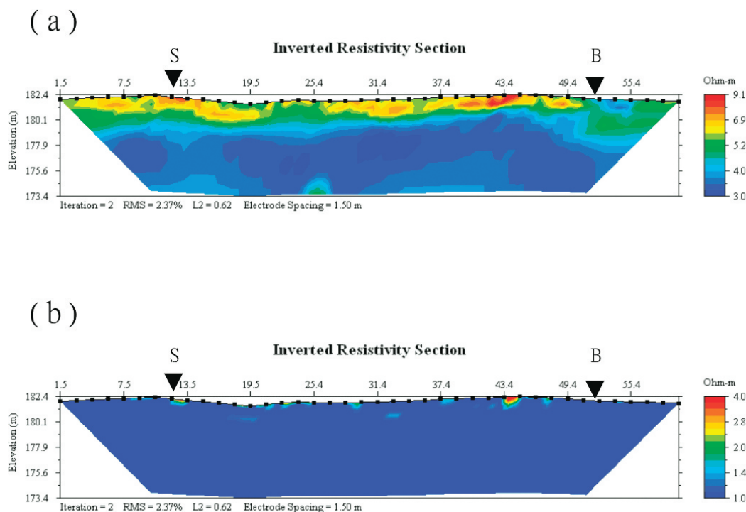
Figure 5. (a) Average resistivity of the hourly surveys along the D line. (b) Standard deviation of resistivity of the hourly surveys along the D line.
