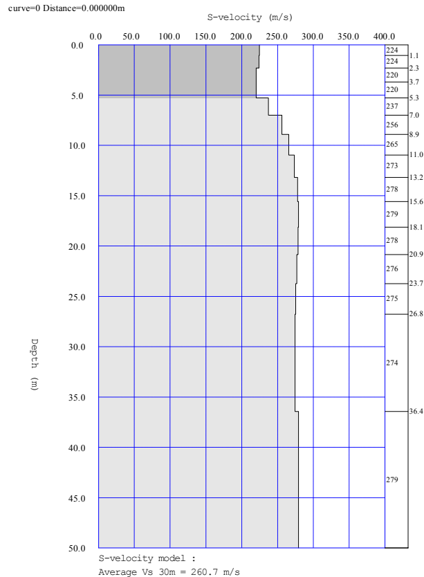
Figure 10: OHC: Shear-wave velocity profile determined using the MASW analysis. NEHRP average Vs100 = 853 ft/sec (~260 m/sec)
