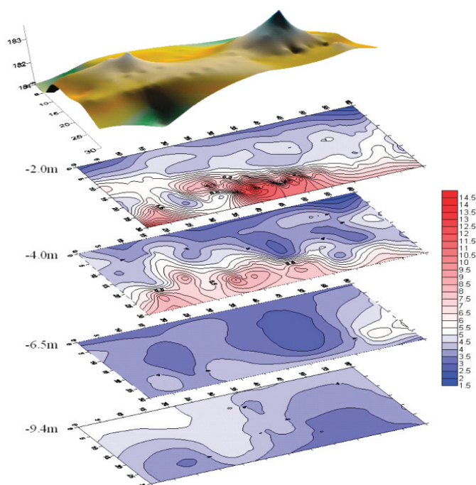
Figure 4. Background resistivity images collected at the WNLPA site in July 2006. The resistivity image of each different depth was created by applying the kriging method to the inversion results from the C, D, E, and F lines and from the X, Y, and Z profiles.
