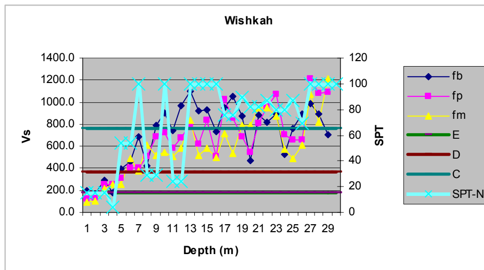
Figure 12: Velocity and SPT-N (blow counts) profiles for the WISH (Wishkah High School) site. Symbols fb, fp and fm represents first break, first peak and first maximum, respectively, arrival times of the shear waves vibrating transversely to the source-receiver (radial) direction.
