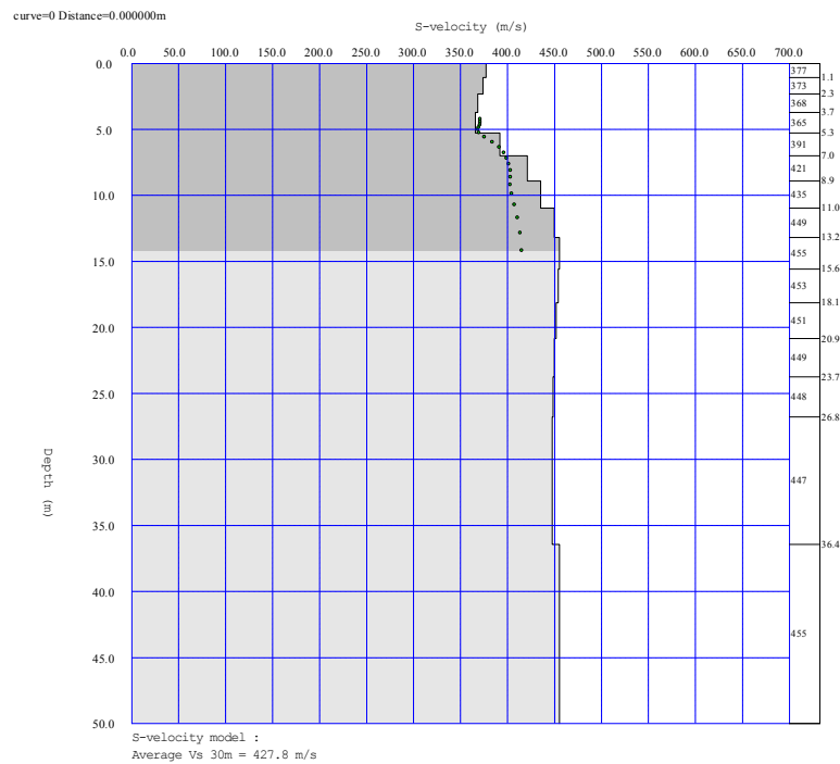
Figure 7: Shear velocity profile obtained from MASW analysis. This velocity profile gives averaged V_{s100} = 1403 ft/sec.
