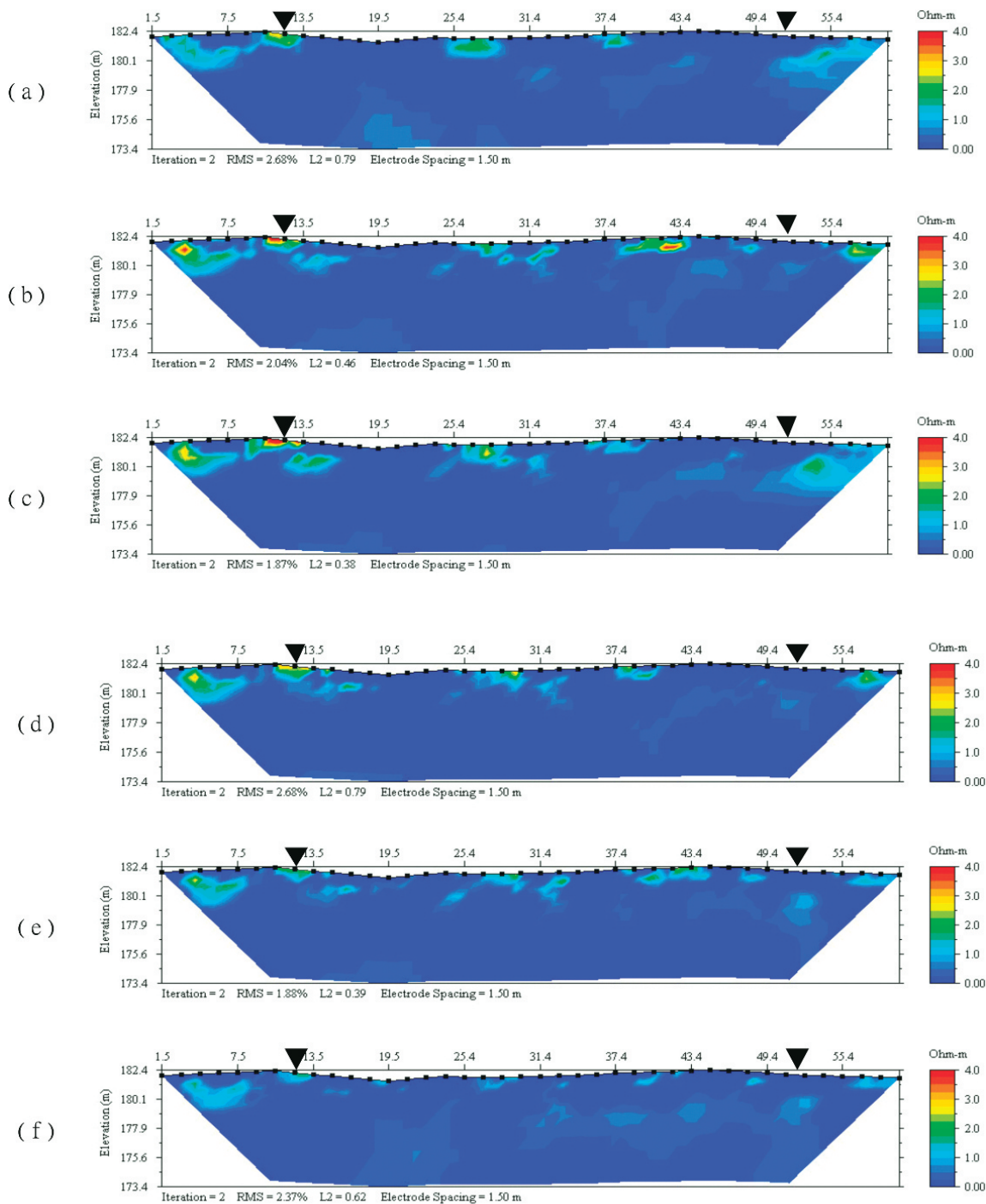
Figure 6. Resistivity difference in the background data collected at (a) day 2, (b) day 3, (c) day 4, (d) day 5, (e) day 6, and (f) day 7 in the 7-day observation study.
