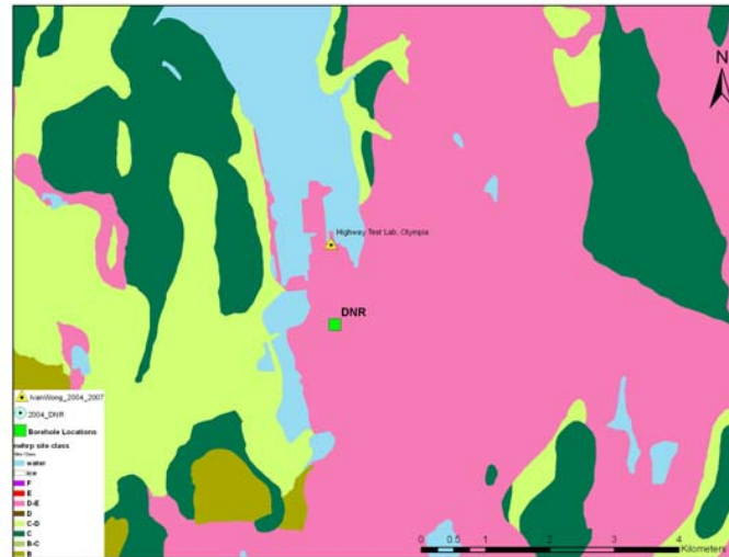
Figure 2: DNR site is underlain by NEHRP site class map (Palmer et al, 2004) for WA. The site was previously determined as NEHRP class D-E.
