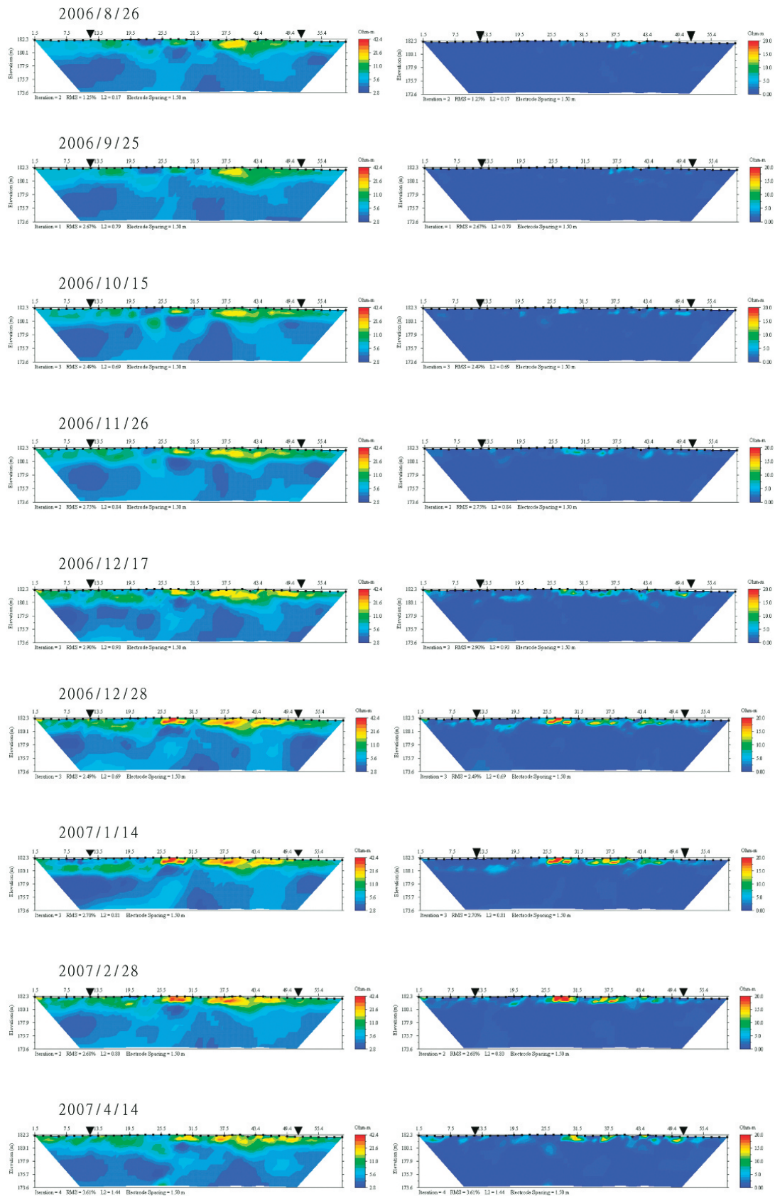
Figure 8. Left: the inverted resistivity images of the E line for long-term monthly observations. Right: the resistivity difference of the E line with respect to the background data (July 22, 2006).
