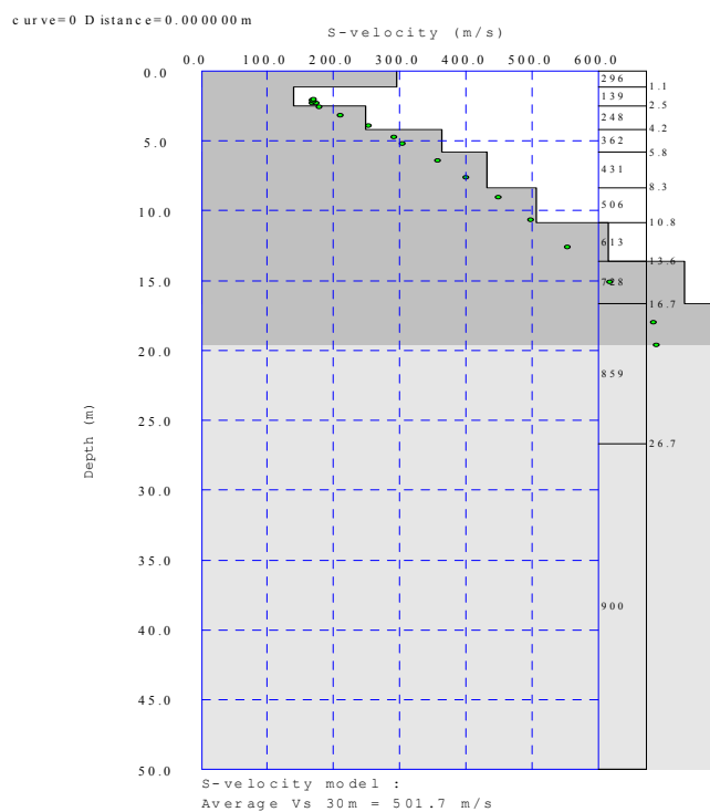
Figure 13: WISH: Shear-wave velocity profile determined using the MASW analysis. NEHRP average Vs100 = 1646 ft/sec (~502 m/sec).
