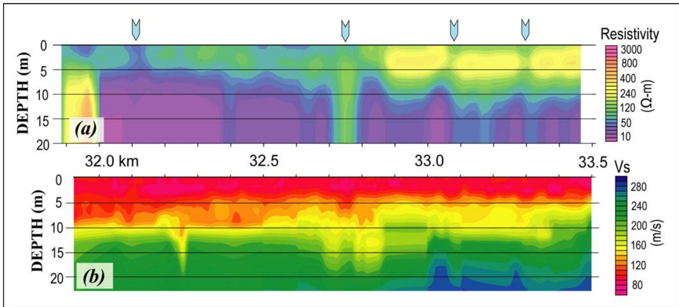
Figure 5. Comparison of survey profiles along Kokai_32L100 line. (a): Resistivity profile inverted from OhmMapper data. (b): S-wave velocity profile calculated from MASW survey data. Uppermost part down to 4 to 5 m deep corresponds to the levee body.
