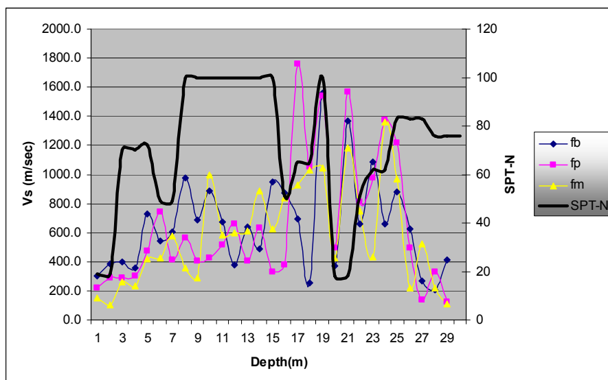
Figure 6: Velocity and SPT-N (blow counts) profiles for the RRHS (Rochester) site. Symbols fb, fp and fm represents first break, first peak and first maximum, respectively, arrival times of the shear waves vibrating transversely to the source-receiver (radial) direction.
