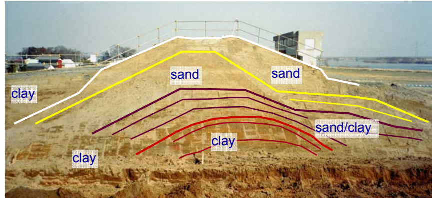
Figure1. A photo showing stacked structure in a levee body revealed at an open cut site.
