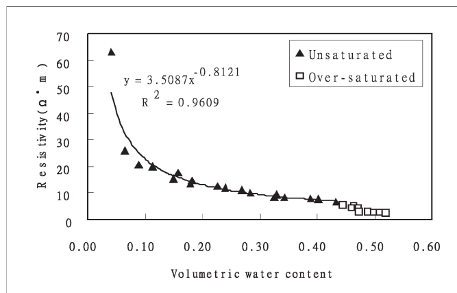
Figure 12. The relationships between the water content and the measured resistivity for the mud samples collected at the area adjacent to the WNLPA site.
