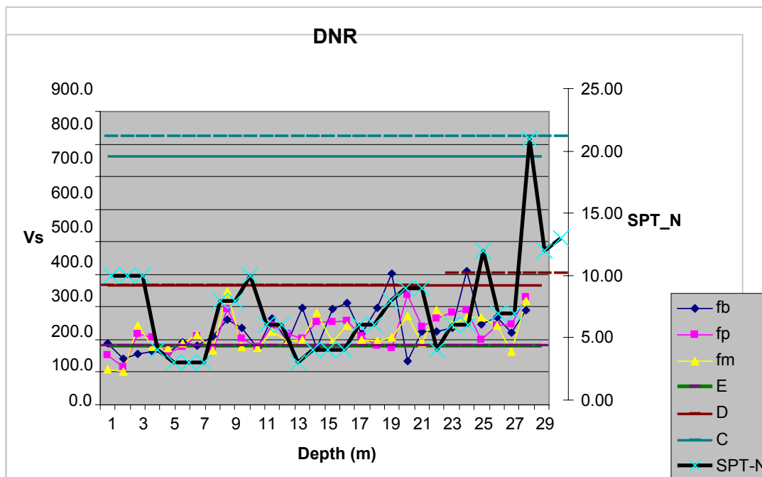
Figure 3: Velocity and SPT-N (blow counts) profile for the DNR site. Symbols fb, fp and fm represents first break, first peak and first maximum, respectively, arrival times of the horizontally polarized shear waves. E, D and C lines are marked to identify NEHRP site class boundaries given in the IBC 2006.
