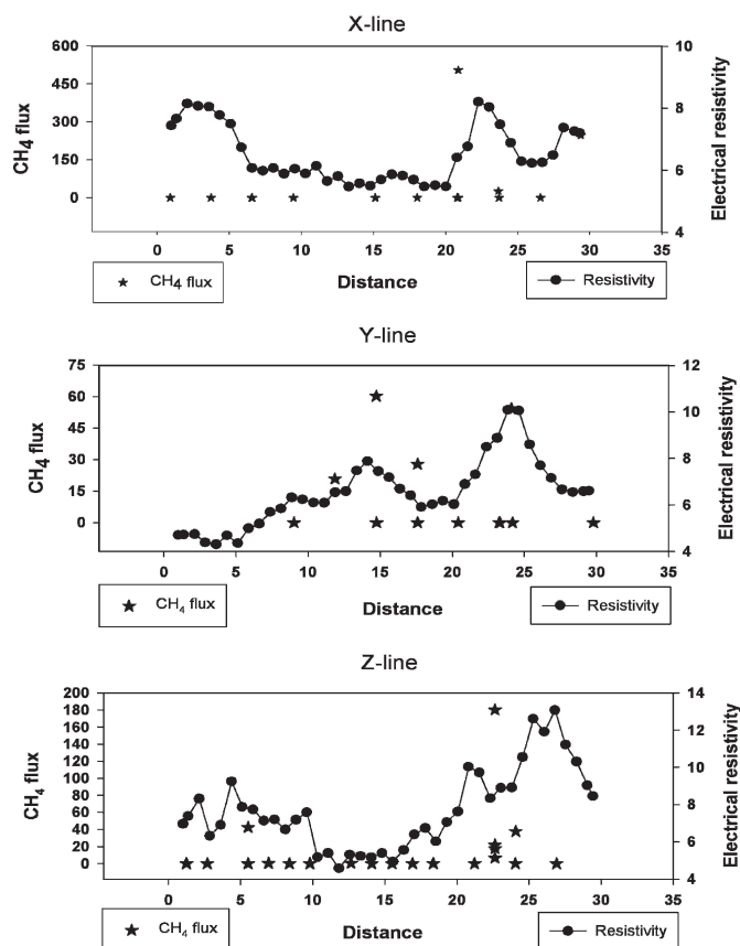
Figure 11. Spatial distribution of 2-D electrical resistivity at a depth of 1.2 m and micro-seepage of CH 4 flux measured by Hong et al. (2009) in the WNLPA. Methane flux measurements close to X, Y, and Z lines were projected on those profiles for comparison.
