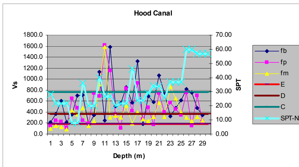
Figure 9: Velocity and SPT-N (blow counts) profiles for the OHC (Hood Canal) site. Symbols fb, fp and fm represents first break, first peak and first maximum, respectively, arrival times of the shear waves vibrating transversely to the source-receiver (radial) direction.
