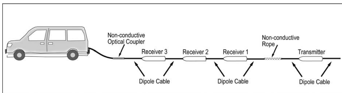
Figure 3. Schematic illustration of the OhmMapper tool.
