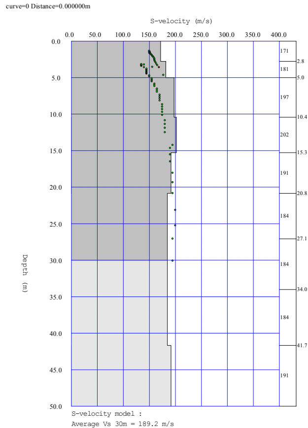
Figure 4: V_s velocity profile determined from the MASW analysis. This profile gives 620 ft/sec for the NEHRP average velocity ( V_{s100} ) of top 100-feet soil column.
