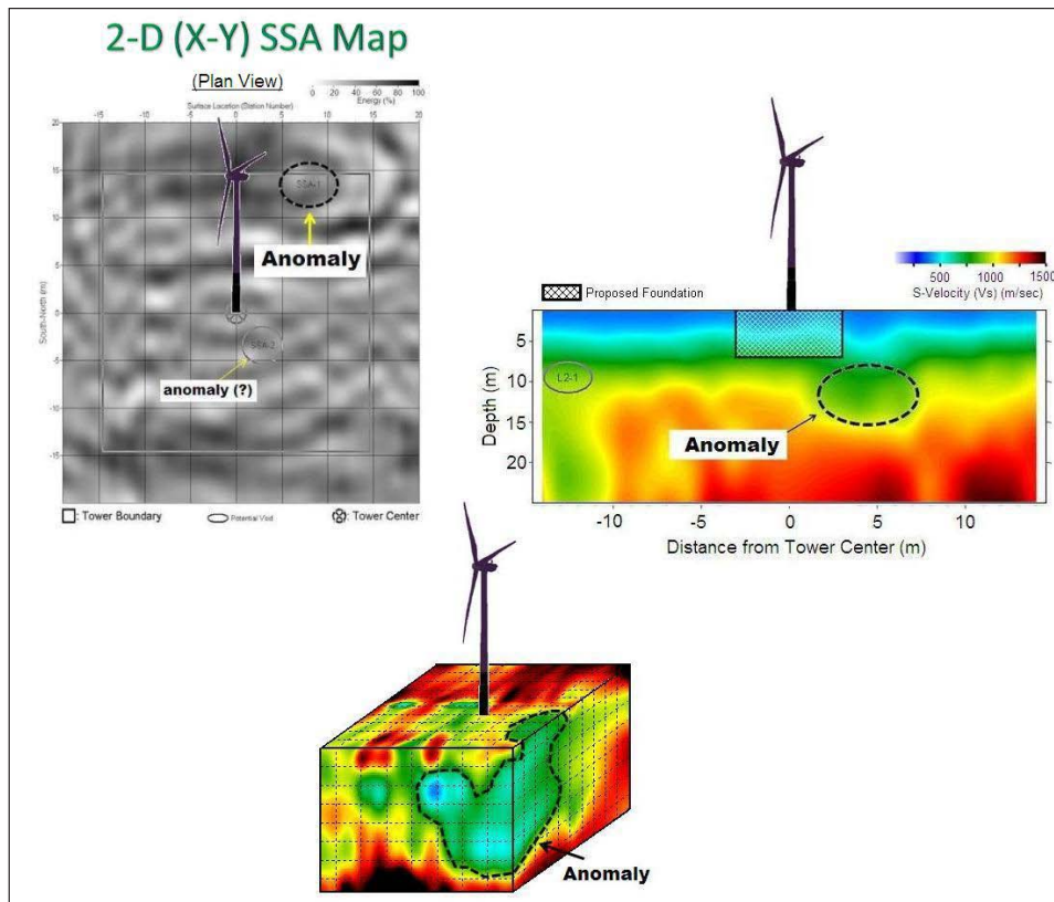
Figure 8. Side-scattering-analysis (SSA) map (upper left), 2-D Vs map (upper right), and 3-D Vs map showing a potential anomaly at a proposed turbine site in a Midwest state.
