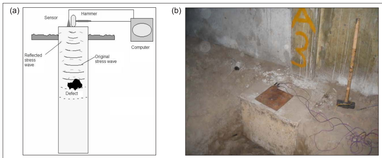
Figure 3. (a) Schematic of pulse-echo test; (b) system components.
