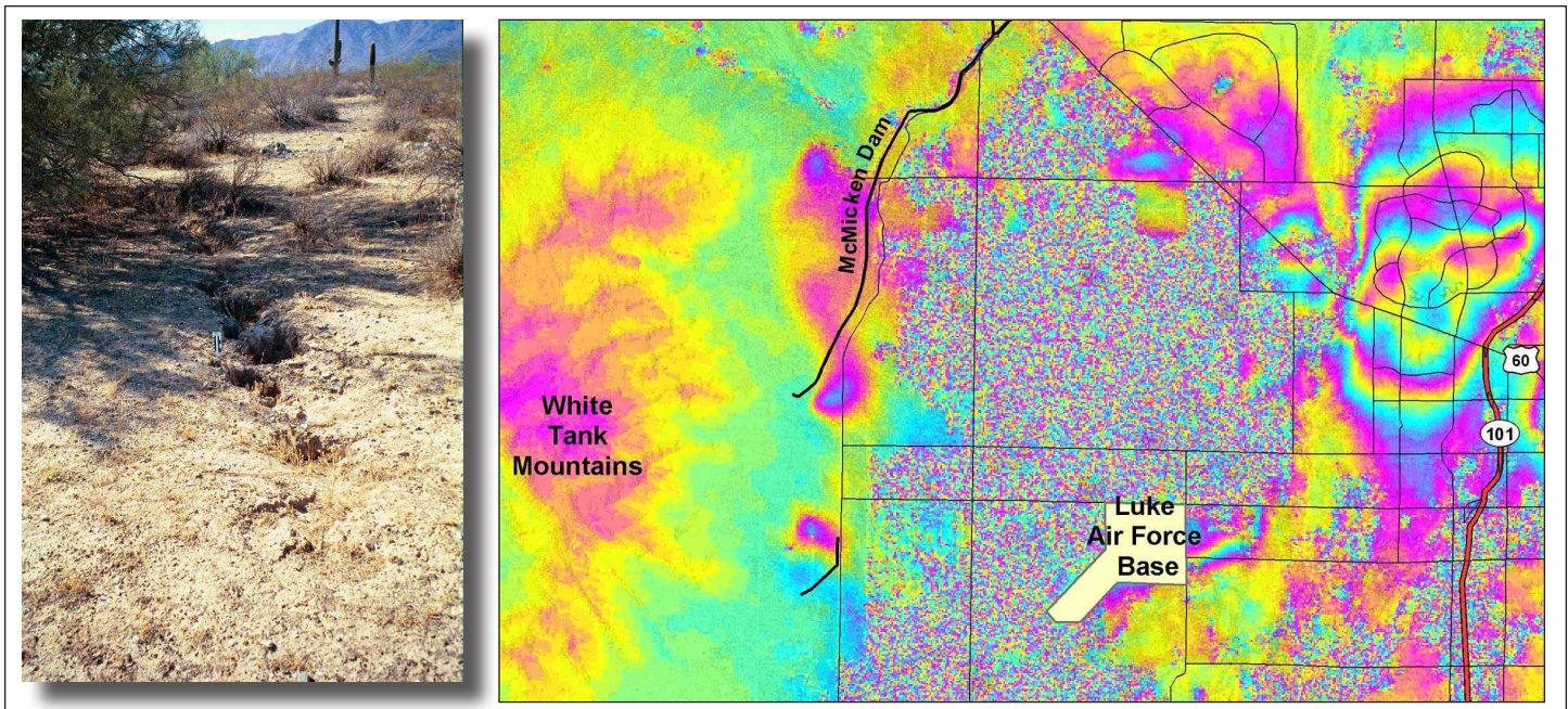
Figure 1. An earth fissure with surface expression of piping erosion (left), and a 32-km-wide InSAR image (ADWR, 2003) depicting relative land subsidence in the western Salt River Valley west of Phoenix, Arizona from December 1996 to 1999. Differential elevation change is presented as color change; a complete color cycle, such as blue to blue or yellow to yellow, represents 3 cm elevation change over the 3 years. General subsidence is apparent in Sun City, Arizona in the northeast corner of the image, and immediately east of Luke Air Force Base. Distinct subsidence bowls are apparent at the south end of McMicken Dam and at White Tanks No. 3 FRS about 3 km to the south.
