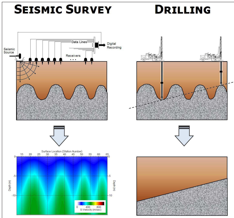
Figure 4. Advantage of seismic surveys in comparison to conventional drilling.
