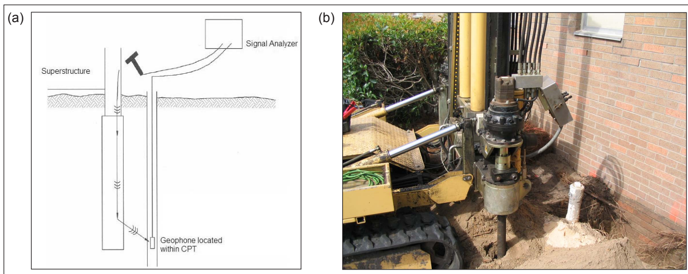
Figure 5. (a) Schematic of parallel seismic testing; (b) parallel seismic test using seismic CPTu.
