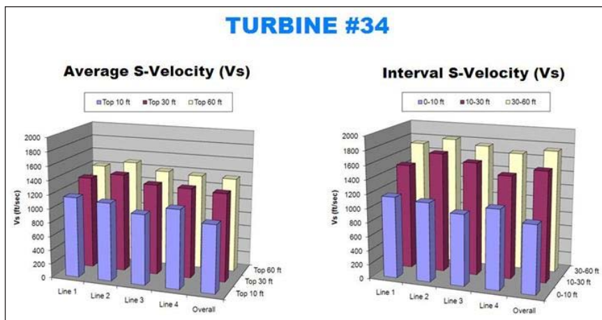
Figure 6. Display of average and interval shear-wave velocities for four (4) lines surveyed at a proposed turbine site in a Midwest state.
