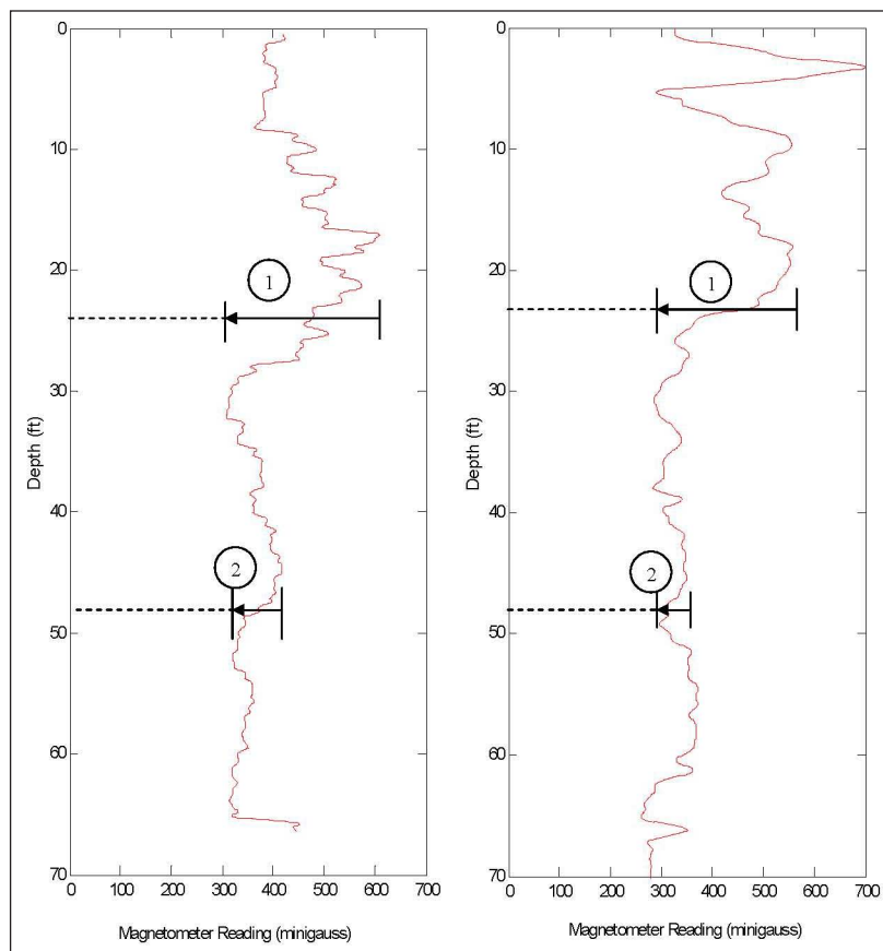
Figure 8. Magnetometer reading with depth at column A3 (left) and A19 (right).
