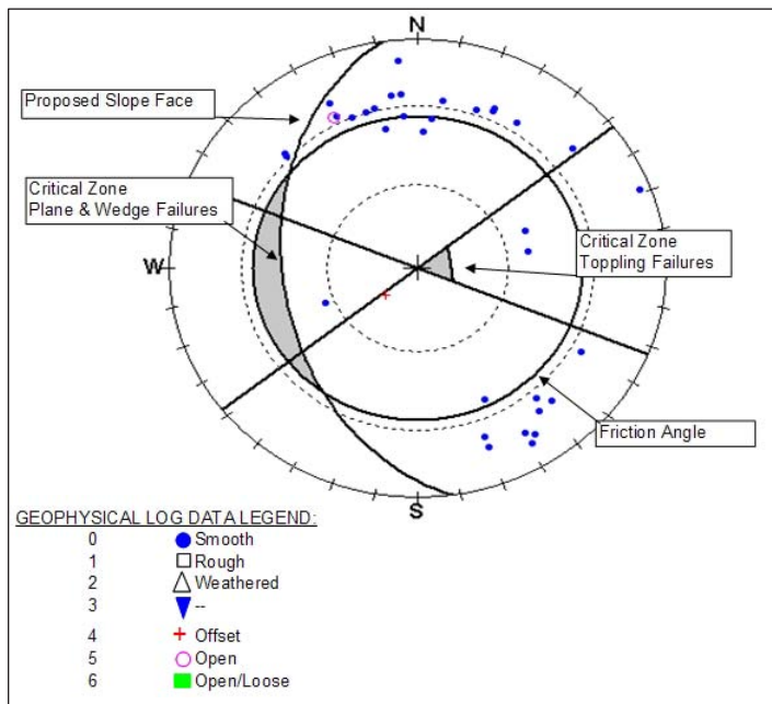
Figure 5. Rockpack III stereonet representation of Markland's Test for identification of rock slope failures using borehole geophysical data.
