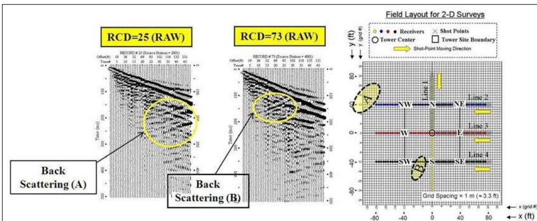
Figure 10. Anomalies (A and B) identified from the back-scattering features on field records and corresponding locations on the field map.
