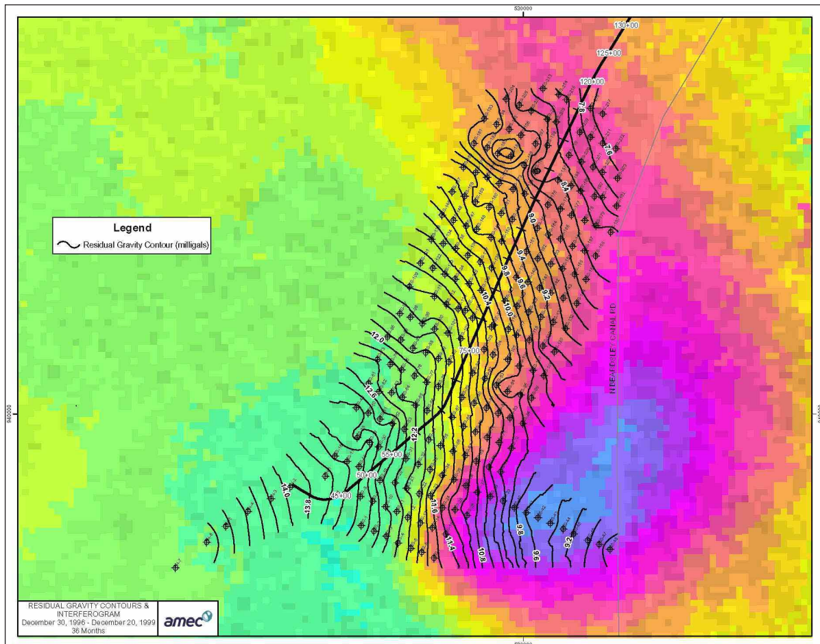
Figure 3. Southern end of McMicken Dam and gravity survey overlaid on InSAR interferogram showing distribution of subsidence between 1996 and 1999. Nearly 3 cm of relative elevation change is indicated from the south end of the dam to the center of the subsidence bowl (blue is at bowl center) to the east. Gravity survey began on bedrock southwest of the dam. About 1.8 miles of dam is shown.
