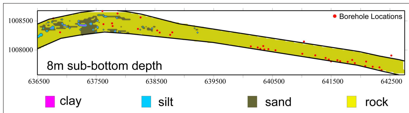
Figure 7. Example of material type conversion from a depth slice at 8 m below the canal floor.
