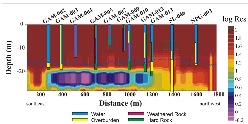
Figure 5. Example of co-located borehole and resistivity data on the Gamboa region. Borehole drilling spans from 1943 to the present and indicates water levels at the time of drilling which in many cases was before current canal floor dredge depths (blue line).
