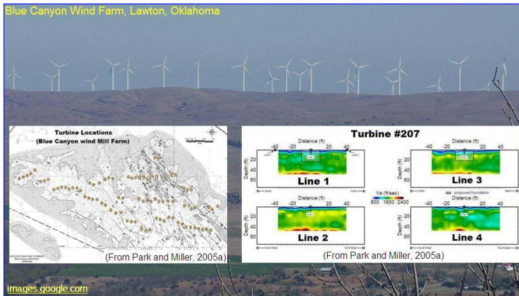
Figure 2. Blue Canyon Wind Farm near Lawton, Oklahoma, a turbine location map, and an example of multiple 2-D shear-velocity ( V_s ) profiling at one turbine site (from Park and Miller, 2005a).
