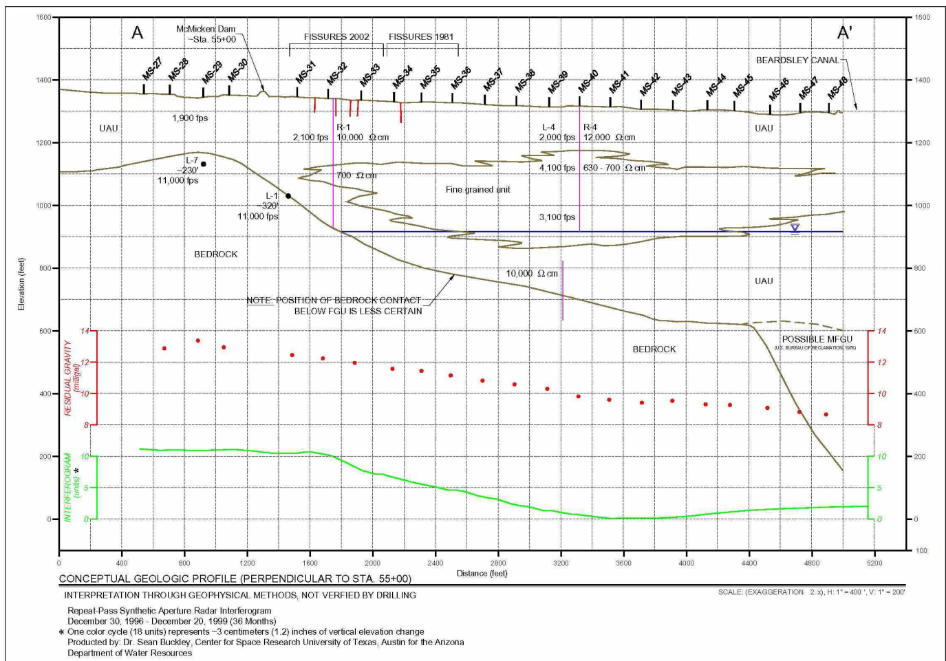
Figure 4. Conceptual basin profiles based primarily on surface geophysics were used to develop finite-element coupled-seepage and stress-strain models to assess current and potential future subsidence and ground-strain conditions (Weeks and Panda, 2004) for dam mitigation, including abandonment of part of the existing dam and design of new dam section.
