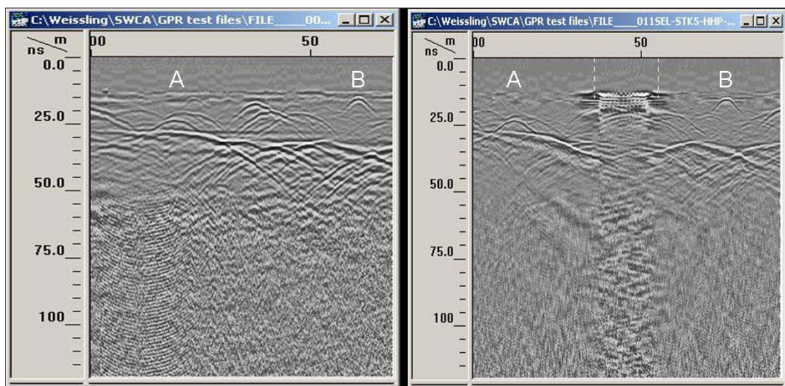
Figure 2. Radargrams (200 MHz) of an evaluation of microwave attenuation/transmission effects of a wire mesh at the antenna-ground coupling position. For positional reference, features A and B (diffraction hyperbolas) are identified in both panels. The dashed vertical lines in the right panel represent the location of the wire mesh sheet.
