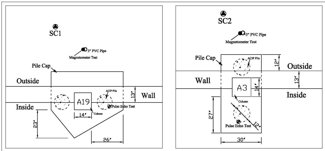
Figure 2. Plane view of columns A3 and A19 and their relationship to locations of drilled shaft.
