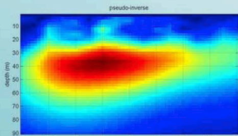
GMR 2D image of relative permeability
