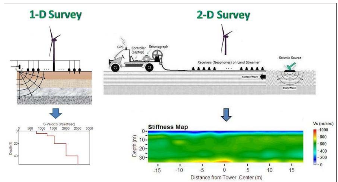
Figure 5. 1-D and 2-D wind-turbine site characterizations by the MASW method.
