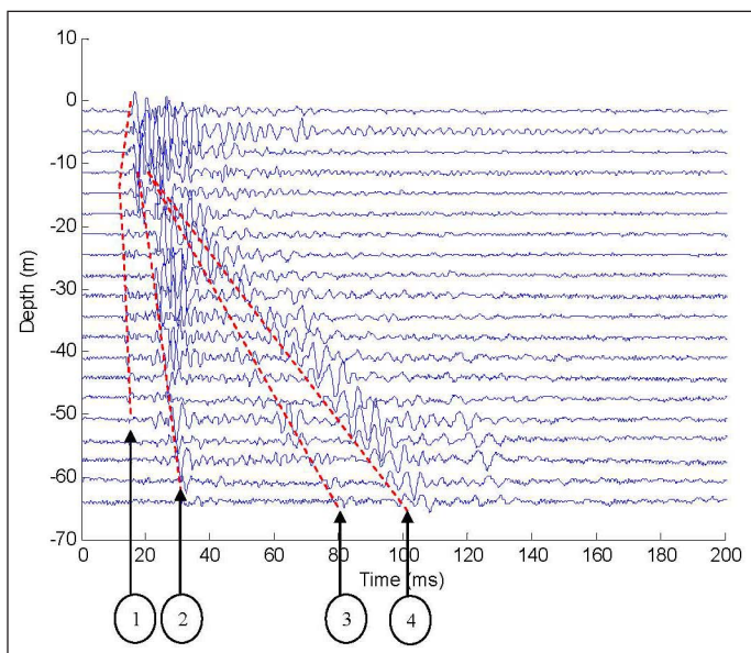
Figure 6. Signals from parallel seismic testing with wave trains identified.
