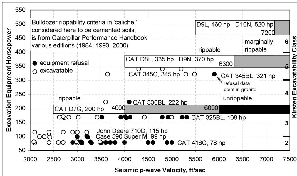
Figure 6. Empirical correlation of backhoe and trackhoe excavation performance in cemented soils in the Salt River Valley area of Arizona at test pits with overlapping seismic lines (modified from Rucker and Ferguson, 2006). The Kirsten (1982, 1988) excavatability classification system (excavatability class on right side of figure) has been adapted to address erodability (Annandale, 1995; NRCS, 2001). These correlations can begin to provide a quantitative empirical link from seismic velocity to erodability.
