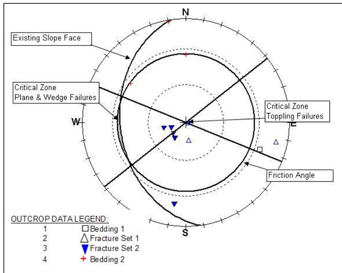
Figure 4. Rockpack III stereonet representation of Markland's Test for identification of rock slope failures using only outcrop data.
