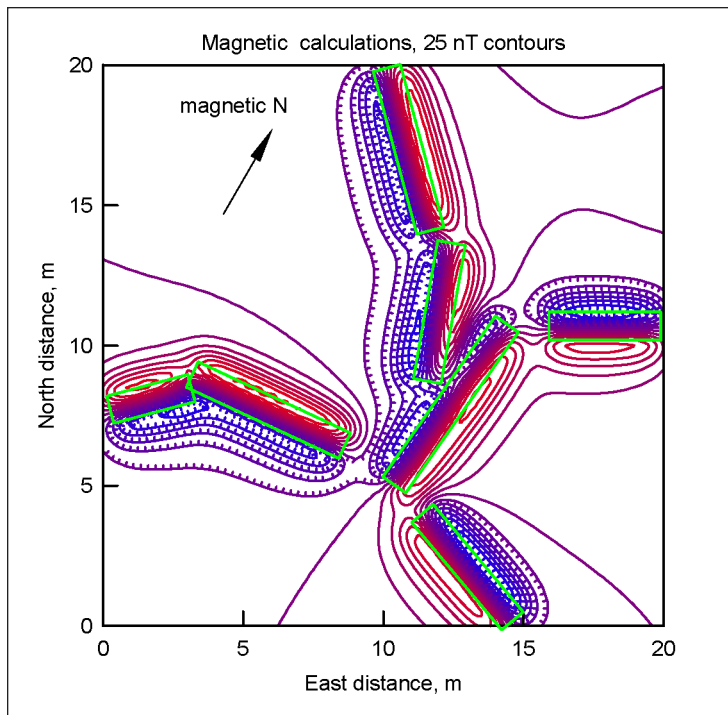
Figure 2. The calculated field of a simple magnetic model. The magnetization in each rectangular slab is horizontal and perpendicular to the length of the slab.
