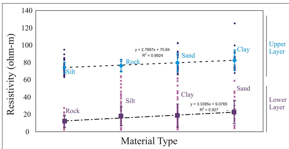
Figure 6. Scatter and regression of material type and electrical resistivity.
