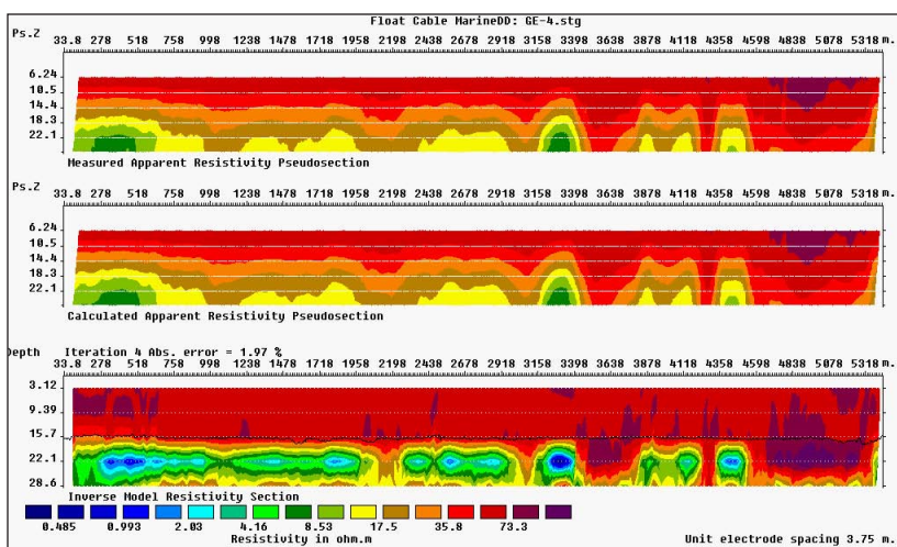
Figure 4. RES2DINV output presentation showing observed apparent resistivity (top), calculated resistivity (middle), and model section (bottom) with a black line indicating depth of water.
