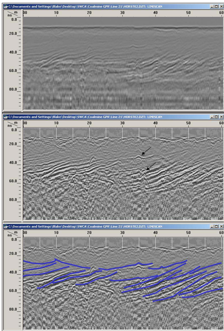
Figure 4. Raw (top panel), post-processed (middle panel), and interpreted (lower panel) radargram (200 MHz) of a 55-m profile of the passage floor. Radar reflections are consistent with sandstone cross-bedding structure. Arrows denote a structural hump and possible disturbance area (diffraction hyperbola).
