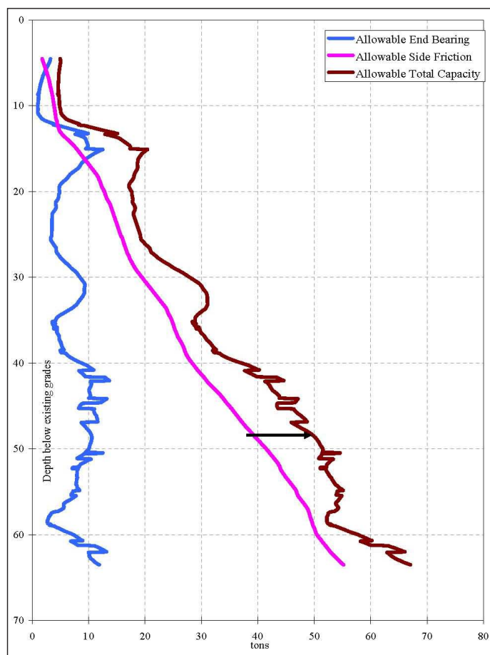
Figure 9. Pile net bearing capacity with depth using French method.
