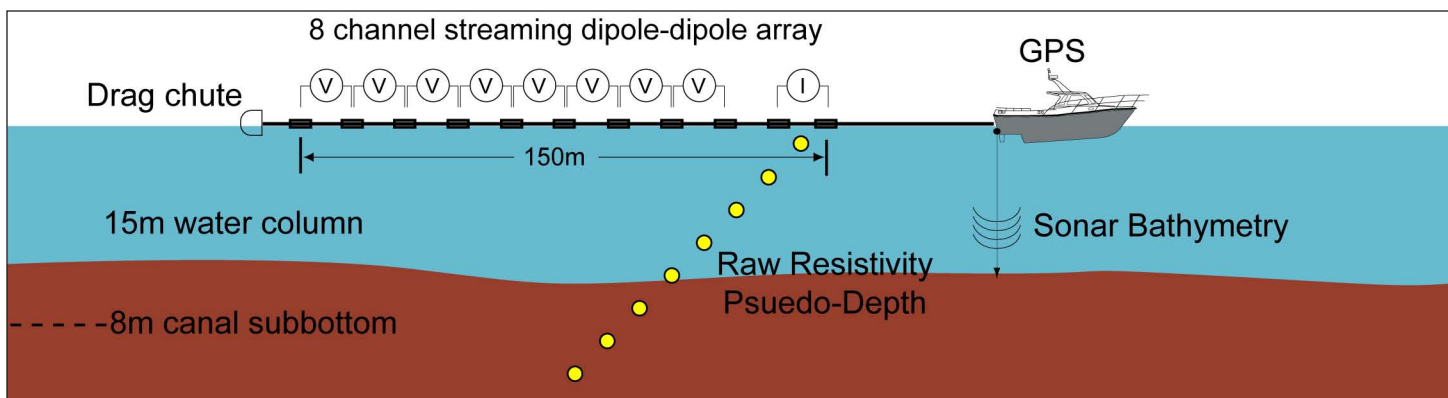
Figure 3. Schematic of streaming marine resistivity system.
