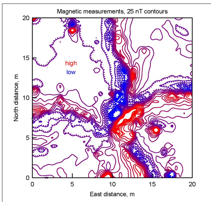
Figure 1. Total magnetic field in a 20-m square. Four radial arms are apparent in the measurements; each linear high is clockwise from a low.
