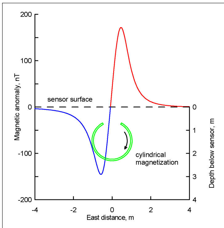
Figure 3. The magnetic anomaly of a cylindrical shell. The magnetization is cylindrical, as marked by the arrow in the cross-section of the model. Note that the upper part of the cylinder is missing.
