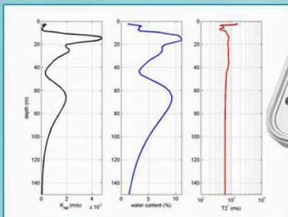
GMR 1D aquifer profile
