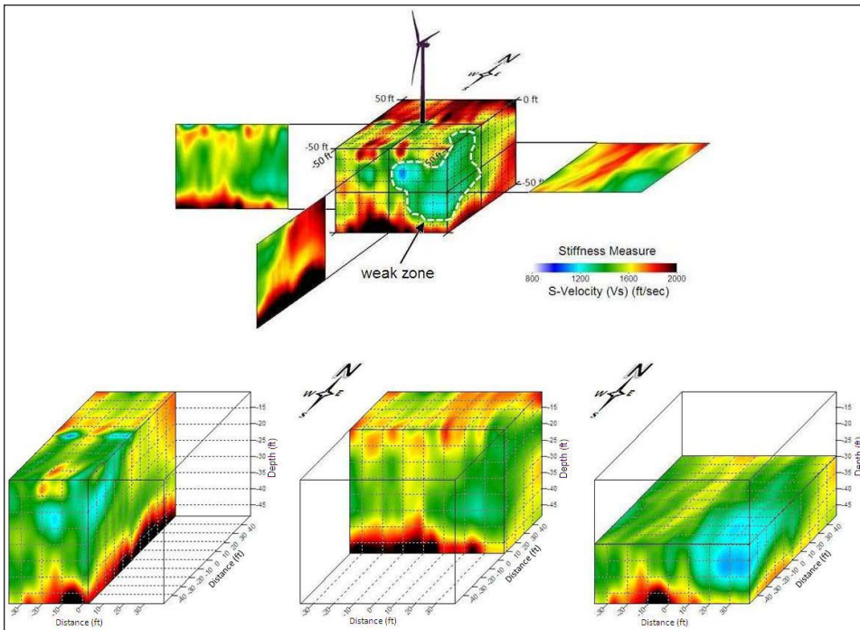
Figure 9. 3-D shear-velocity ( V_s ) mapping of a proposed wind-turbine site in a Midwest state displayed in cubic and layer-slice modes (top) and layer-stripping modes along three orthogonal x-y-z axes (bottom).
