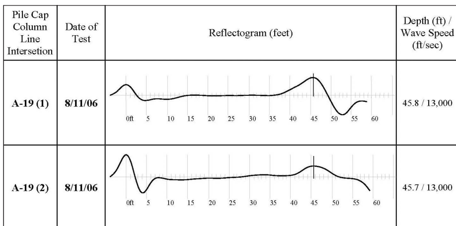
Figure 4. Example of pulse-echo signal after processing.
