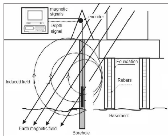
Figure 7. Schematic illustrating use of a magnetometer for pile-length determination.
