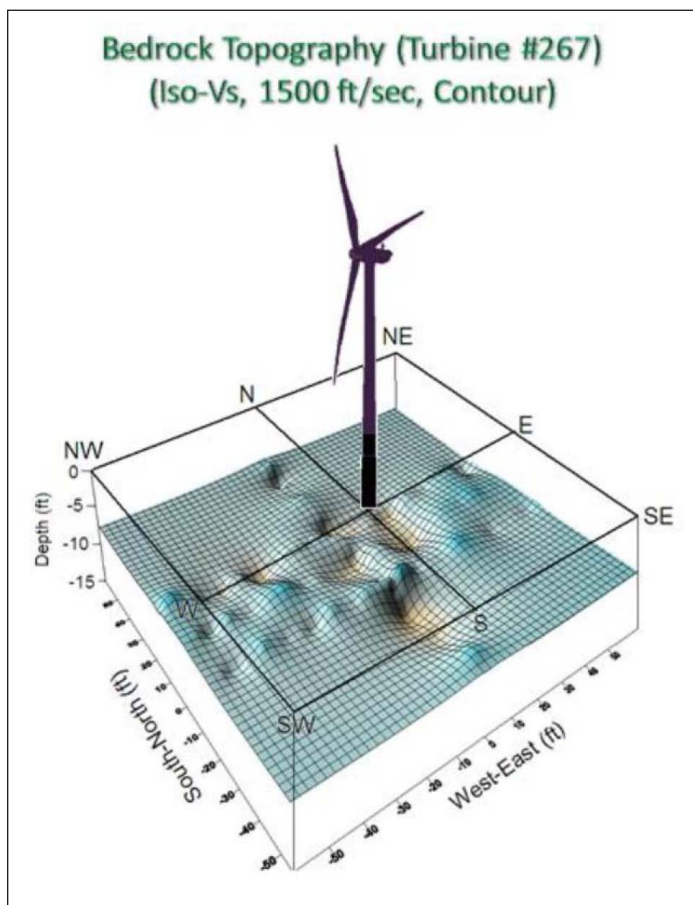
Figure 7. Bedrock topographic map constructed from iso-velocity contouring from four (4) lines of 2-D V_s data at a proposed turbine site in a Midwest state.
