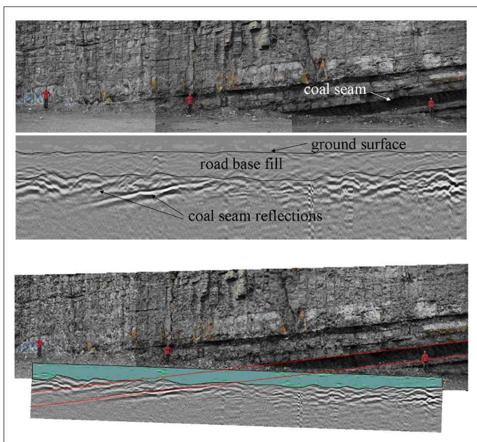
Figure 3. Photo-collage of road cut coal seam and sandstone strata (top panel) with GPR 200-MHz radargram of sub-surface (middle panel). Lower panel depicts registration of photo (stretched to correct perspective) and radargram (compressed vertically to match coal seam inclination). Green layer in radargram depicts road base fill material.
