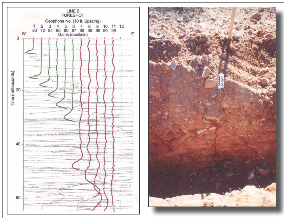
Figure 2. Example seismic refraction traces with used to interpret presence of a possible earth fissure (left), and fissure found in a test pit after being located using seismic method (right). The stake next to the test pit was the marked seismic discontinuity field interpretation. Note that the fissure did not pass through the upper 60 cm of uncemented subsurface material, but was distinct in the underlying cemented horizon.
