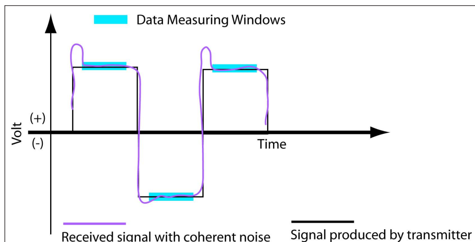
Figure 2. Signal and noise during a marine resistivity survey.
