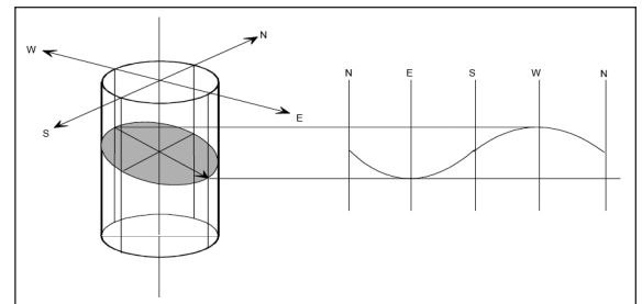
Figure 2. Fracture presentation as sine wave.
