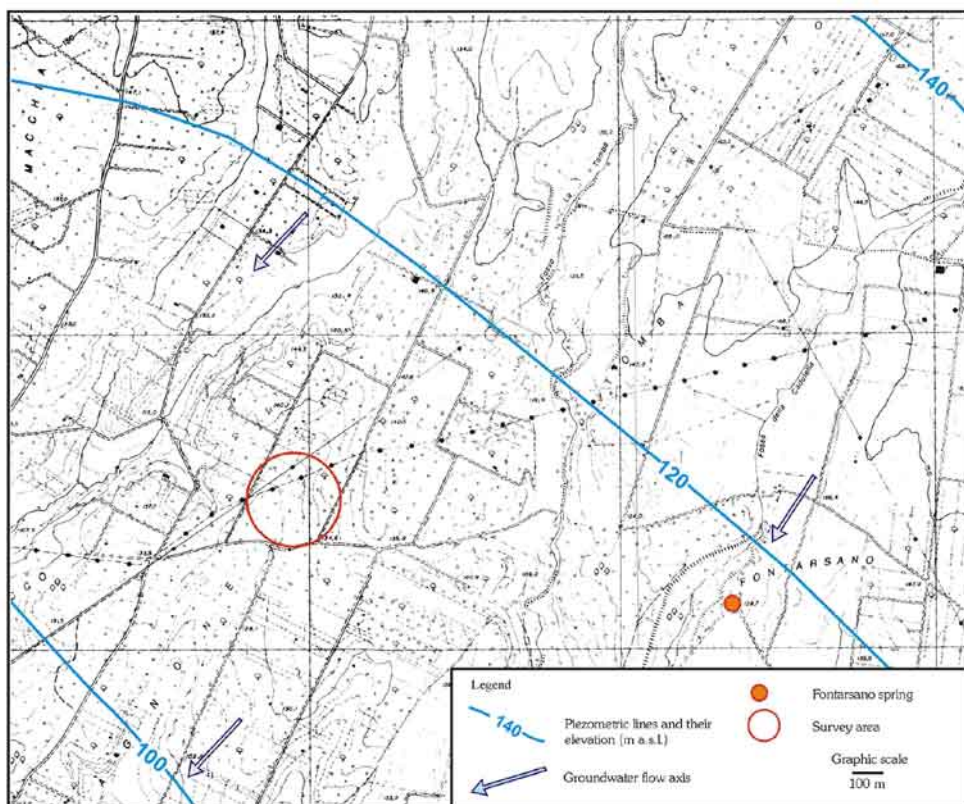
Figure 2. Hydrogeologic map of the survey area.
