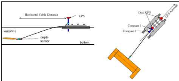
Figure 5. Equipment locations and parameters required for positional calculations.
