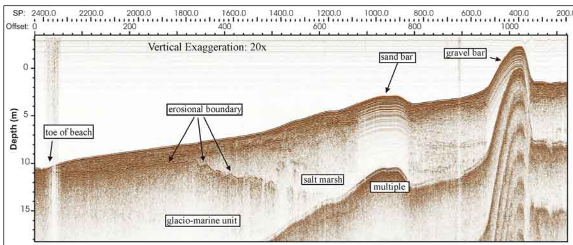
Figure 5. Profile w3000 passing directly over a large gravel bar as shown in Figure 4. The depth scale is referenced to geodetic datum (mean sea level). Vertical exaggeration is 20x.
