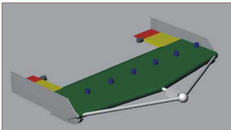
Figure 1. Perspective view of the MTA Sensor Platform showing Cesium magnetometers (blue), stern planes (red), and the wing-shaped body (green).
