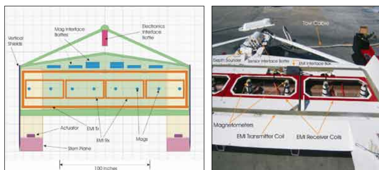
Figure 2. Position of Cesium vapor magnetometers and time-domain EMI transmitter (Tx) and receiver (Rx) coils.
