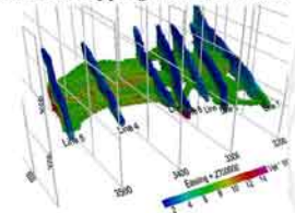
Bedrock Mapping with 3D Seismic
