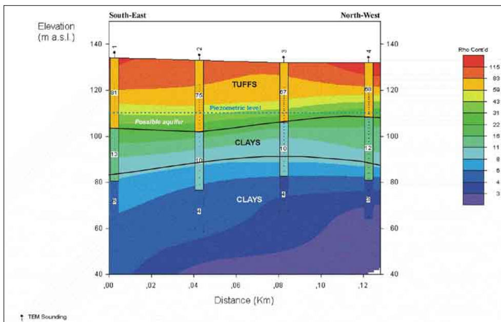
Figure 5. TDEM cross section depicting layered models (columns) and smoothed models (background contouring).
