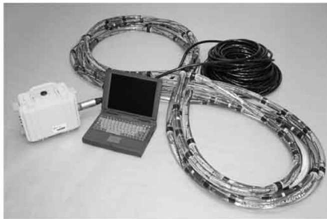
The DHA-6500 connected to a Geometrics GEODE seismograph
