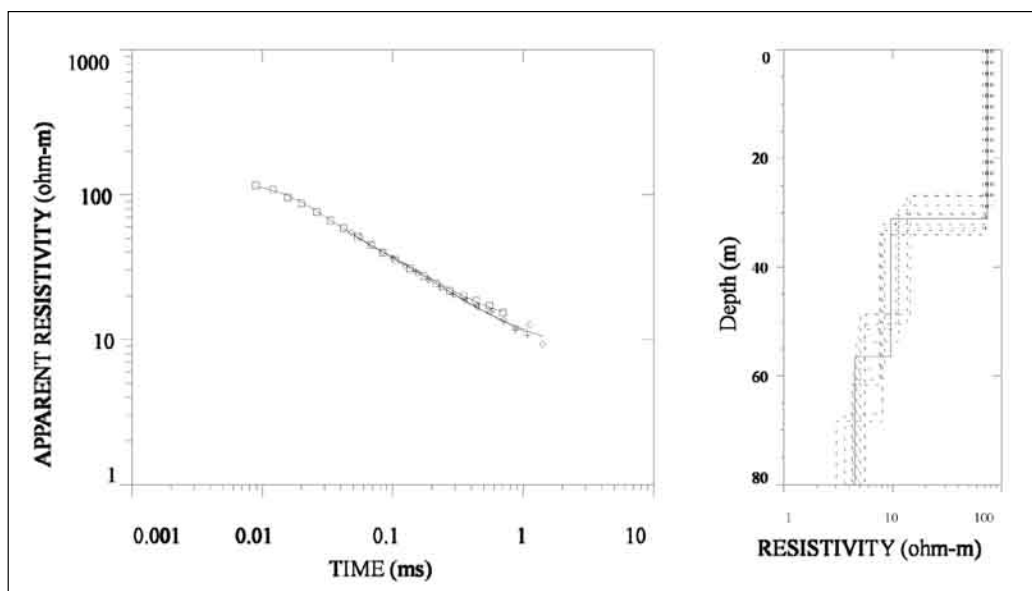
Figure 4. TDEM measurements and models, including the apparent resistivity-time curve (left) and one-dimensional layered models (right). The best-fitting model is shown as a continuous line and equivalent models are shown as dashed lines.
