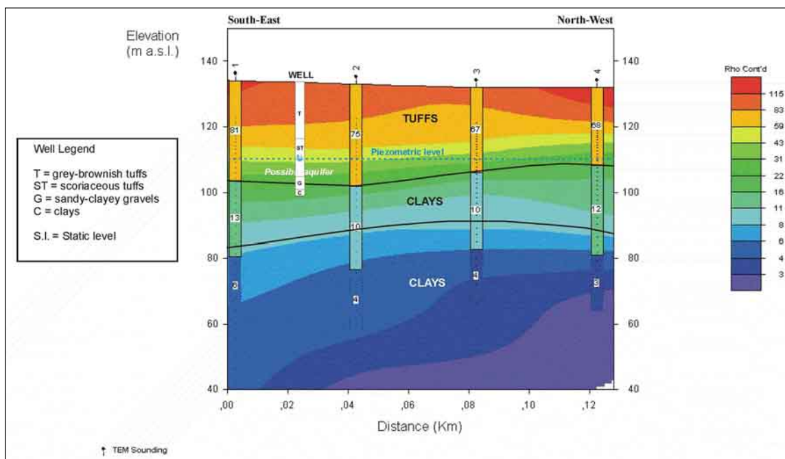
Figure 6. TDEM section including well data.
