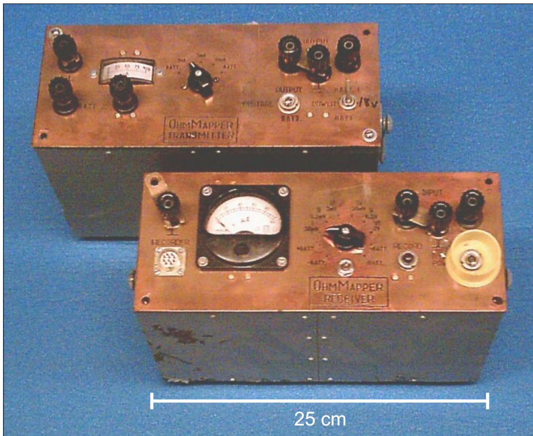
Figure 2. Analog transmitter and receiver of the North American prototype of the Russian-built VCHEP system as delivered to Geometrics. A second copy, shown here, came to the Geological Survey of Canada, and is still in good working order.
